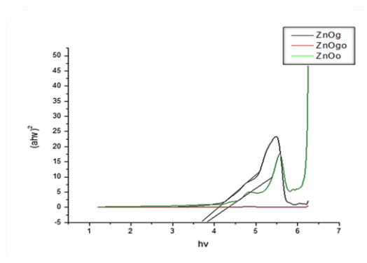
Tauc Plot
