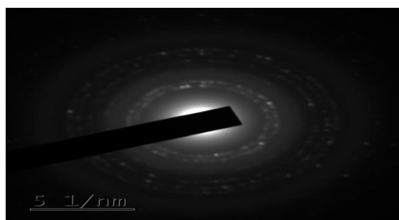
SAED Image
