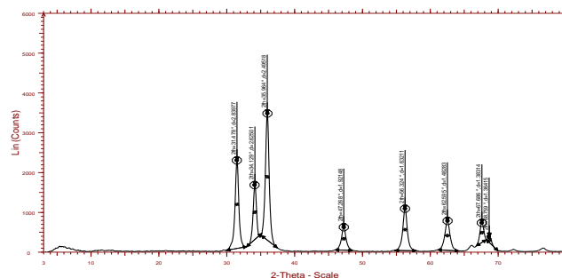
Fig.III: XRD image of ZnO.o NPs
