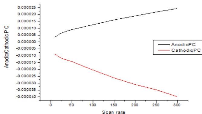
Anodic / Cathodic Peak current at different scan rates in case of ZnO.g+o NP
