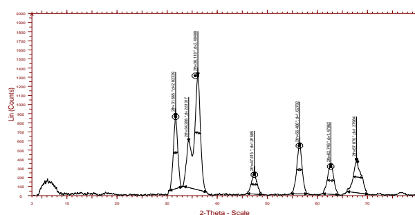
Fig.II: XRD image of ZnO.g+o NPs
