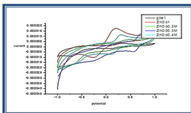
Fig.IXb: CV of ZnO.o NPs in 0.1M, 0.2M, 0.3M and 0.4M K_4Fe(CN)_6 at a scan rate of 0.05V/sec
