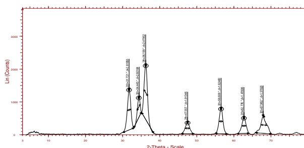
Fig.II: XRD image of ZnO.g+o NPs
